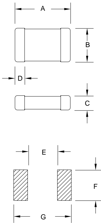
Pad Layout
